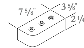
Single Bullnose
