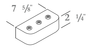
Double Bullnose
